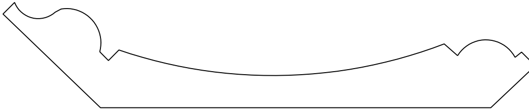
CR21-5.5 1 1/16" x 5 1/2"
